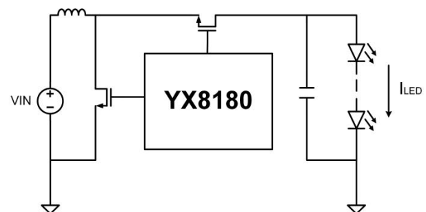
Simplified Circuit Diagram
