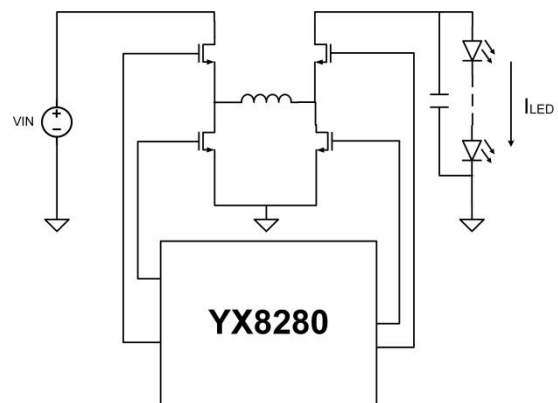
Simplified Circuit Diagram
